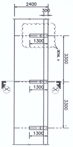
COMPOUND WALL-PLAN (3.0 TO 4.0m HEIGHT)
